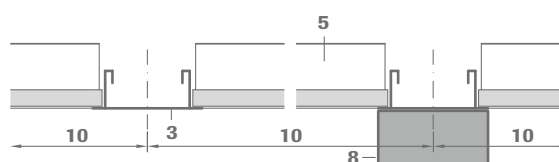
Parallelbandraster
