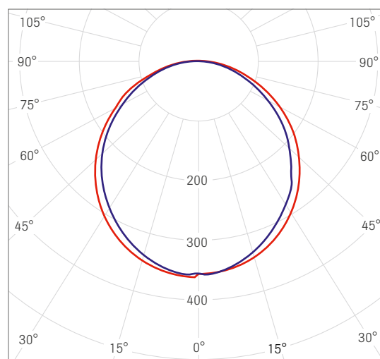
cd/klm n = 100 % — C0 - C180 — C90 - C270
