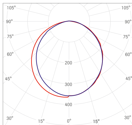
cd/klm — C0 - C180 — C90 - C270 n = 100 %
